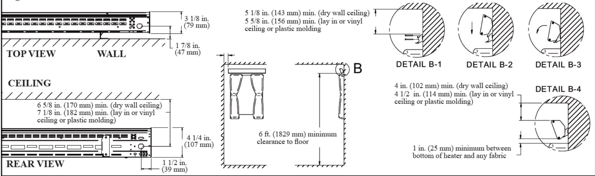
Figure 4 - MOUNTING RESTRICTIONS
