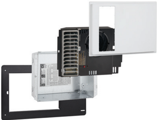
Apex72 heater assembly with accessories shown above. For electronic thermostats sold separately, see page 21
